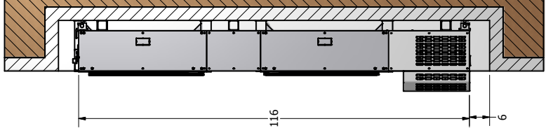
SECTION A-A SCALE 1 / 20
