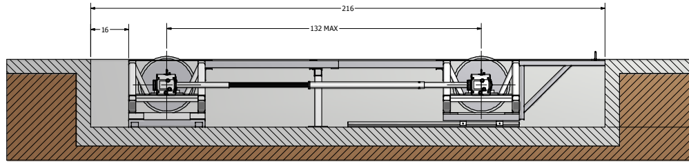
SECTION A-A SCALE 1/18
