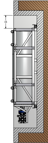
SECTION B-B SCALE 1/18
