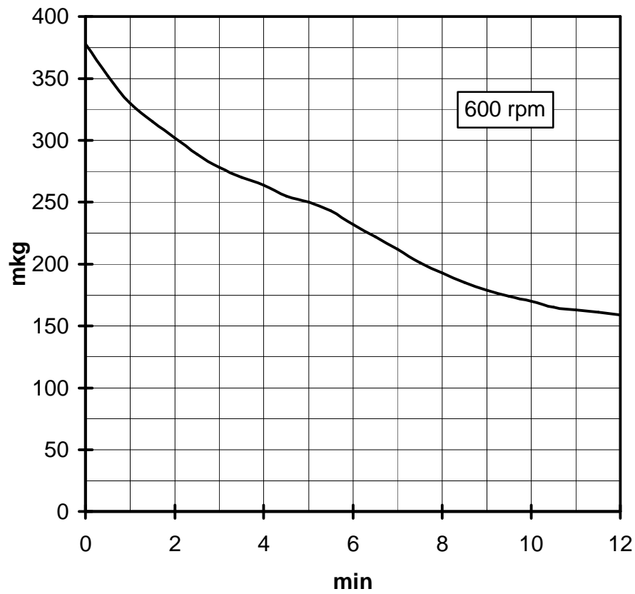
TORQUE vs. TIME
